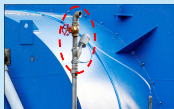
自動清洗裝置氣動入蒸汽閥 Pneumatic steam inlet valve (auto cleaning facility)
